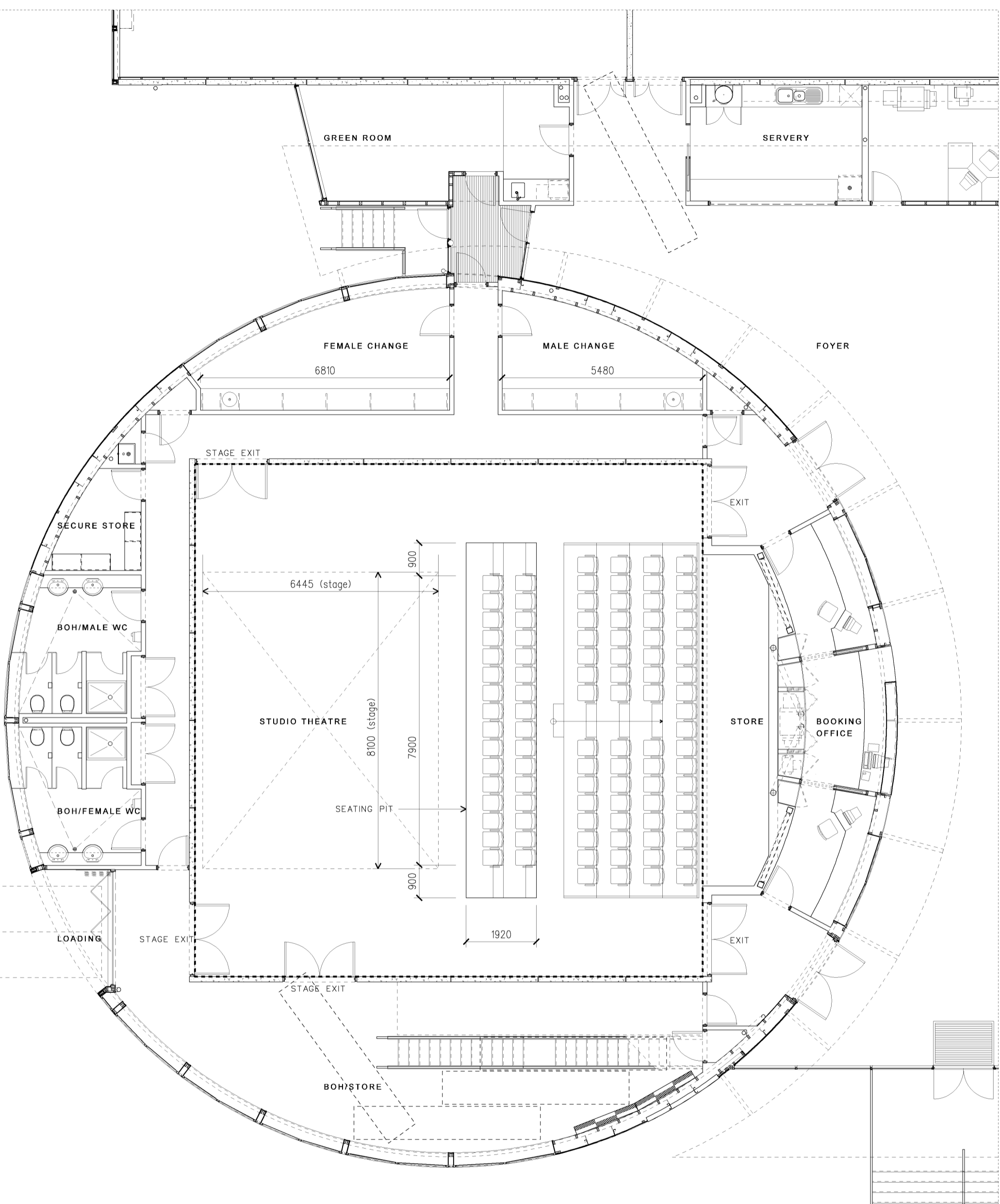
STUDIO THEATRE ROSTRA SEATING - PROSCENIUM MASKING PLAN ROSTRA SEATING PLAN - 98 SEATS
